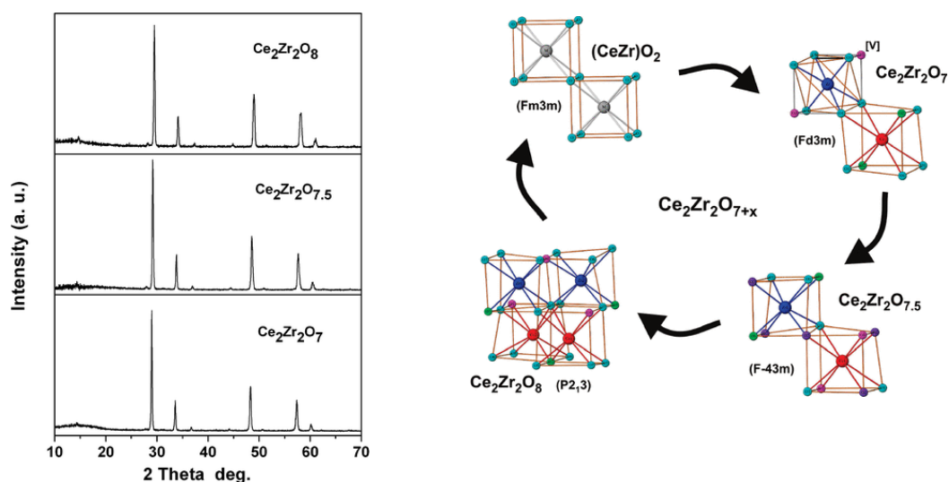
Figure 7.3: (a) Powder XRD patterns and (b) structural transformations in \text{Ce}_2\text{Zr}_2\text{O}_7 , \text{Ce}_2\text{Zr}_2\text{O}_{7.5} , and \text{Ce}_2\text{Zr}_2\text{O}_8 , respectively. (Reproduced from Ref. [10b] with permission of the American Chemical Society).
