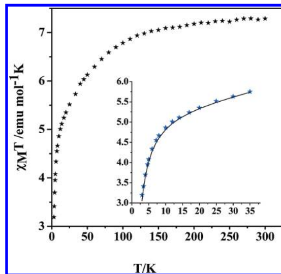
Figure 5. Temperature dependence of the magnetic susceptibility of 1 , in the form of \chi_{\text{M}}T vs T , in the temperature range 3.0–290.0 K using an external magnetic field of 0.5 T. The solid line represents the fitting results (see text).
