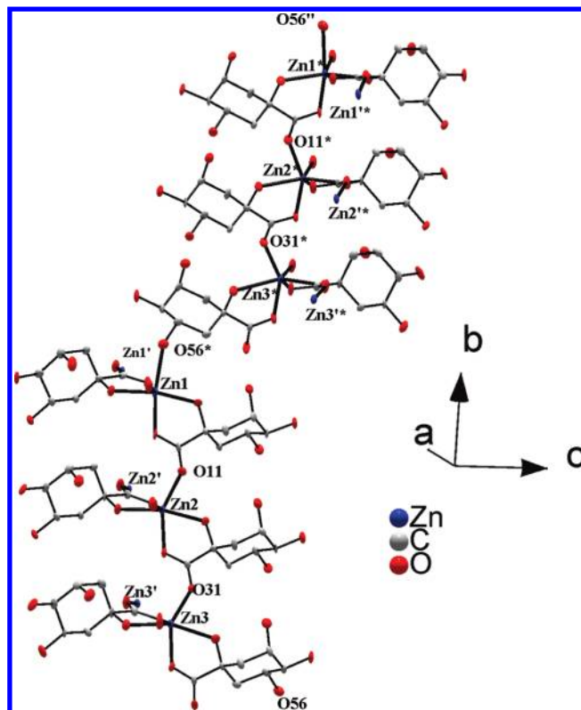
Figure 4. Development of the chain of trimers of 2 along the 2-fold screw axis [2 (0, 1/2, 0) (0.5, y, 0.5)] . Primed atoms are generated by the symmetry operation ( ' ) 1 + x, y, z . Atoms with stars are generated by the symmetry operation ( * ) 1 - x, 0.5 + y, 1 - z .
