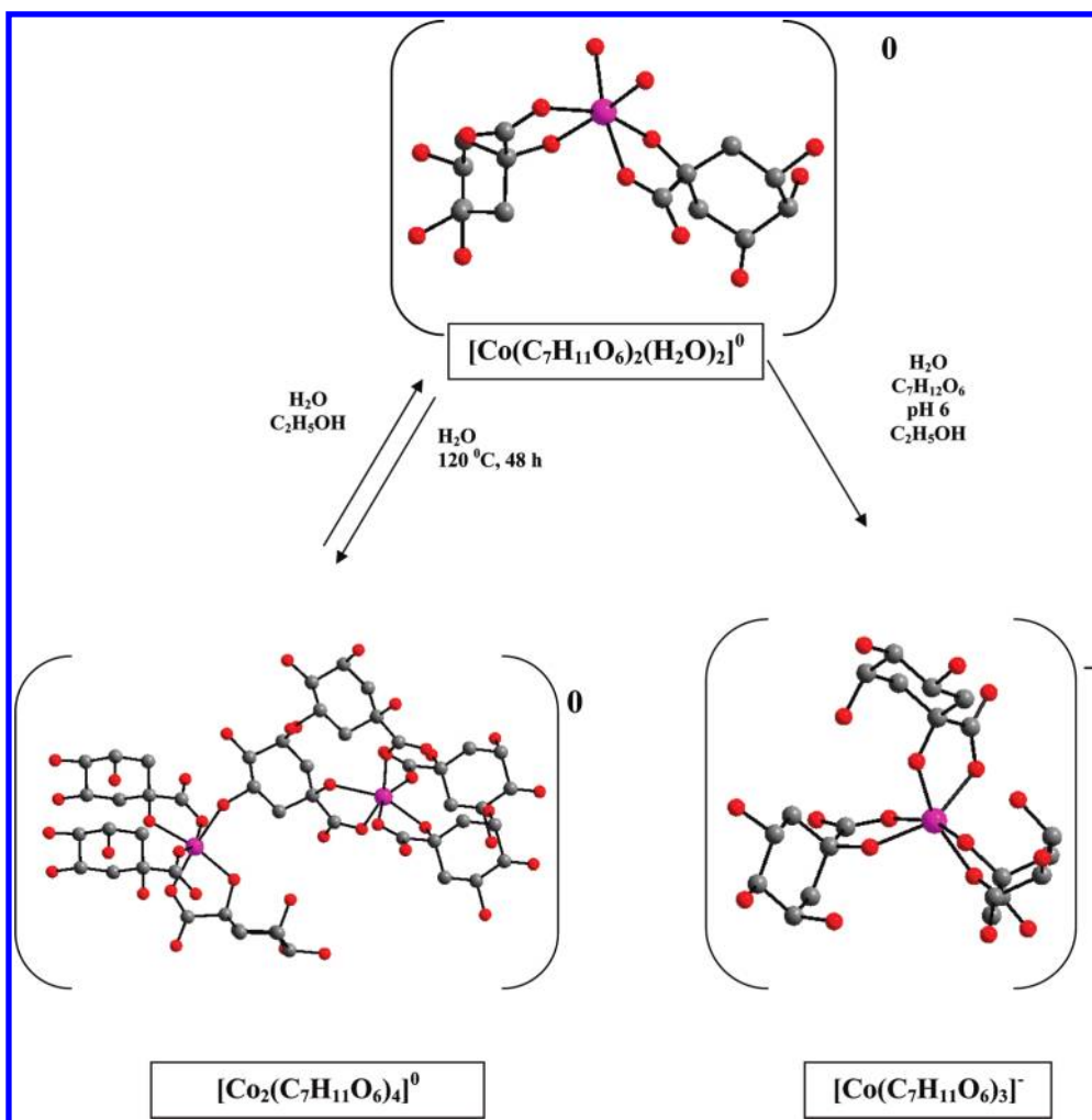
Scheme 1. Transformation Chemistry of the Binary System \text{Co(II)}-\text{D}(-)\text{-Quinic Acid}
