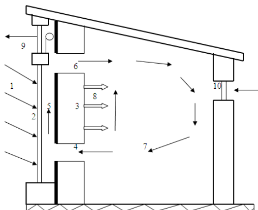
Vertical section of Trombe wall
